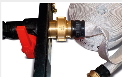
KIT-AIB FIRE-FIGHTING VERSION (EXCEPT FOR 200 L VERSION)
